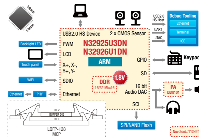
図3: Block Diagram
